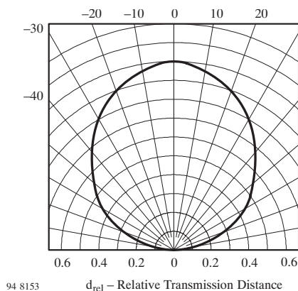
Figure 12. Horizontal Directivity \phi_x
